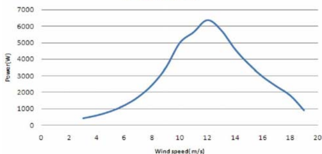
Power curve
